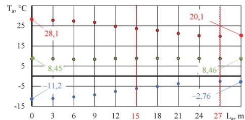
Fig. 15. Graph of experimental dependence between air flow temperature T_a and the path of its movement L_a in a U-shaped vertical-type ground heat exchanger with the air injection of 500\text{ m}^3/\text{h}
