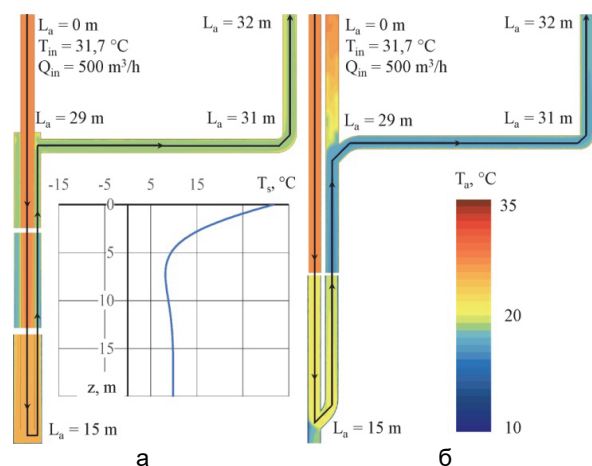
Fig. 7. Temperature field distribution in concentric-type (a) and U-shaped (b) vertical-type ground heat exchangers in summer period with the air injection of 500 m^3/h
