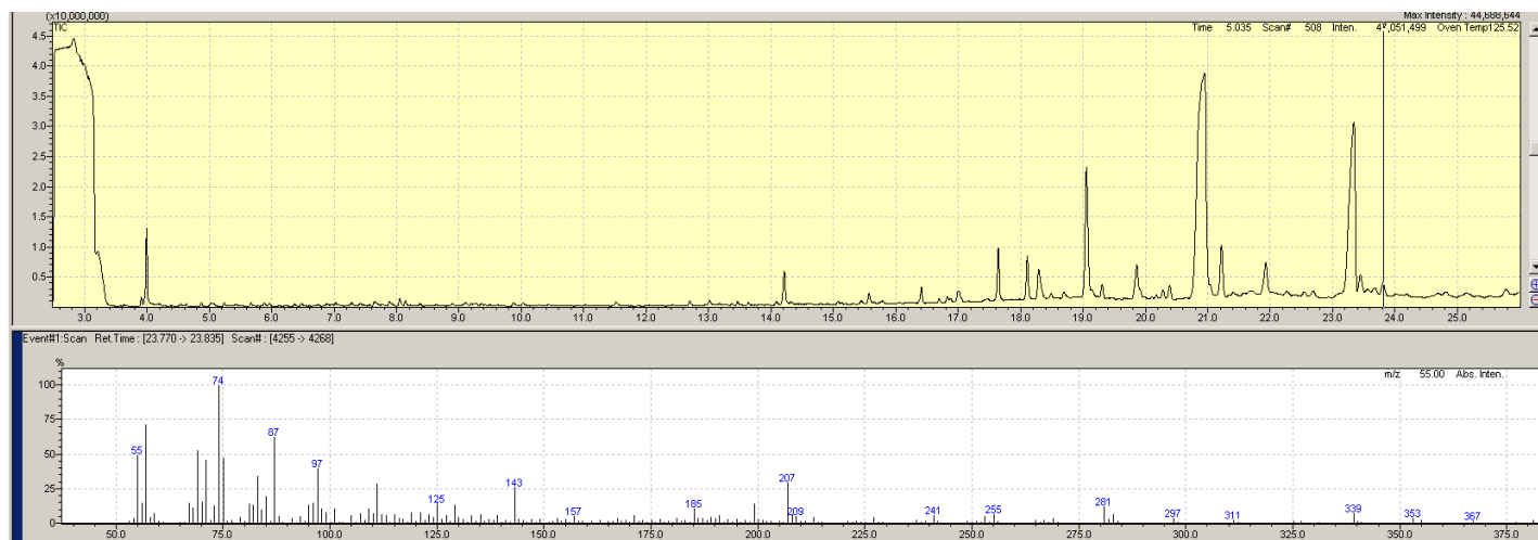
Fig. 1. Chromatogram of GC-MS analysis of the epicuticular wax extracts from the surface of peach fruits (typical distribution of the hydrocarbons for all studied samples)
