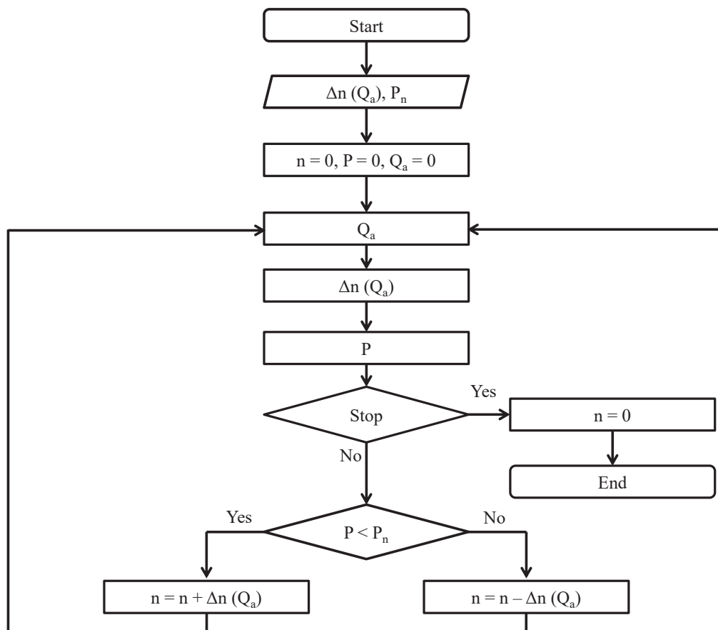
Fig. 8. Algorithm of the servo control system of a rotary plate vacuum pump
