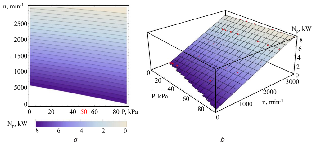
Fig. 6. The influence of rotor speed n and vacuum pressure value P on the power consumption of the vacuum pump drive N_p : a – contour plot; b – three-dimensional plot
