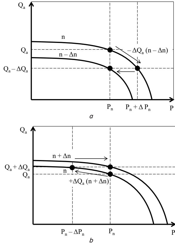
Fig. 3. Changing the mode parameters of the rotary plate vacuum pump during the operation of the servo control system: a – reducing the rotational speed; b – increasing the rotational speed
