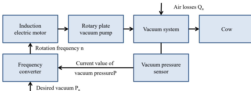
Fig. 2. Technological scheme of a servo control system of the rotary plate vacuum pump of a milking machine
