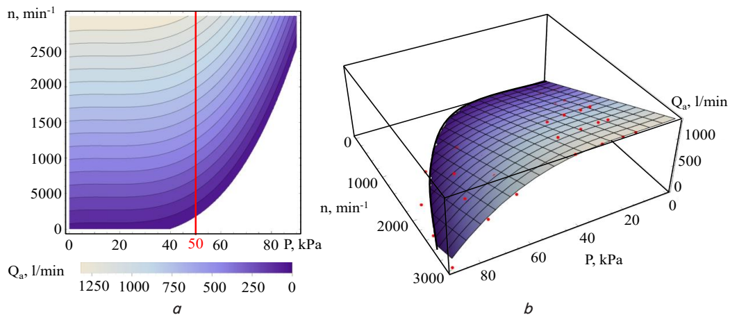
Fig. 4. The influence of rotor speed n and vacuum pressure P on vacuum pump performance Q_a : a – contour plot; b – three-dimensional plot
