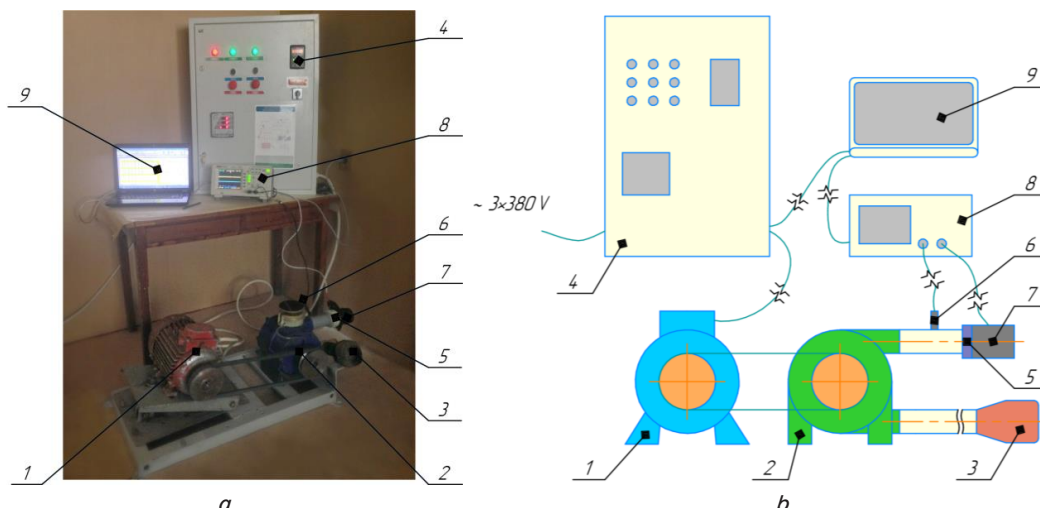
Fig. 1. Experimental bench to study the designed vacuum pump HB-1200: a – general view; b – technological scheme: 1 – induction electric motor; 2 – experimental sample of the rotary plate vacuum pump HB-1200 (Ukraine); 3 – muffler; 4 – frequency regulator Danfoss VLT MicroDrive (Germany); 5 – air flow rate regulator; 6 – pressure sensor MPX5100D (Netherlands); 7 – air flow rate sensor BOSCH 0 280 218 037 (Germany); 8 – RIGOL DS1022C oscilloscope (People’s Republic of China); 9 – personal computer
