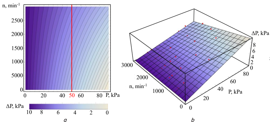
Fig. 5. The influence of rotor speed n and vacuum pressure value P on vacuum pressure fluctuation \Delta P : a – contour plot; b – three-dimensional plot
