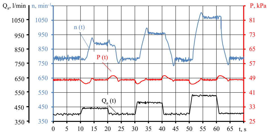
Fig. 10. Dynamics of changes in vacuum pressure P and rotor speed of vacuum pump n when changing air flow rate Q_a of a milk vacuum system of the milking machine for the developed algorithm
