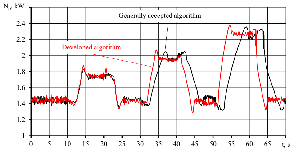
Fig. 11. Dynamics of changes in the power of the vacuum pump drive N_p for the proposed algorithms
