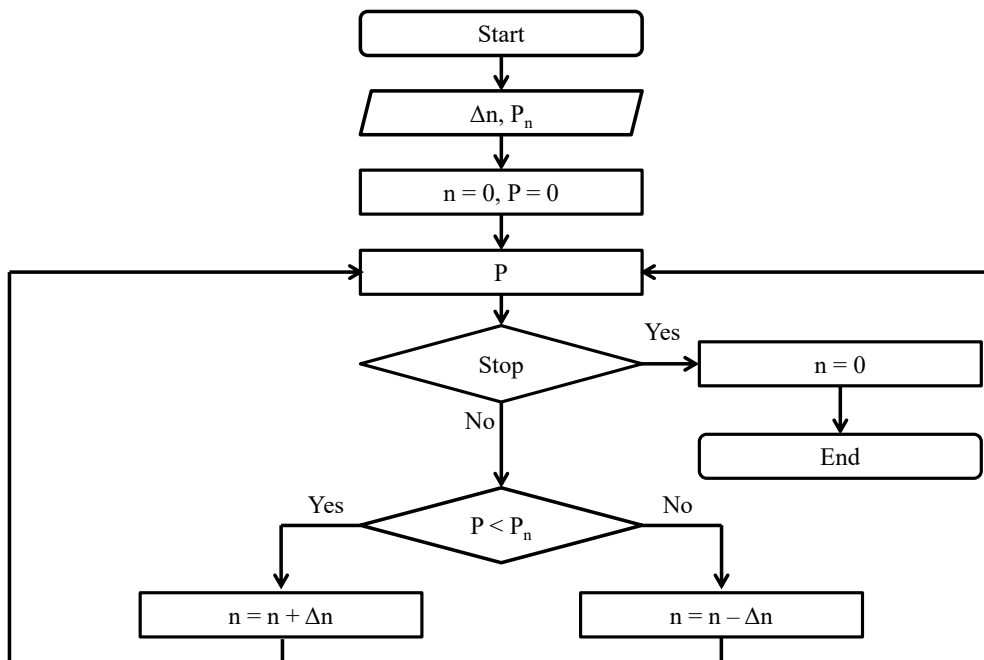
Fig. 7. Generally accepted algorithm for the servo control system of a rotary plate vacuum pump
