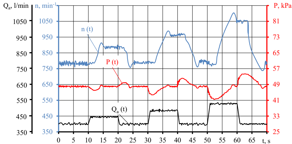
Fig. 9. Dynamics of changes in vacuum pressure P and rotor speed of vacuum pump n when changing air flow rate Q_a of a milk vacuum system of the milking machine for the generally accepted algorithm
