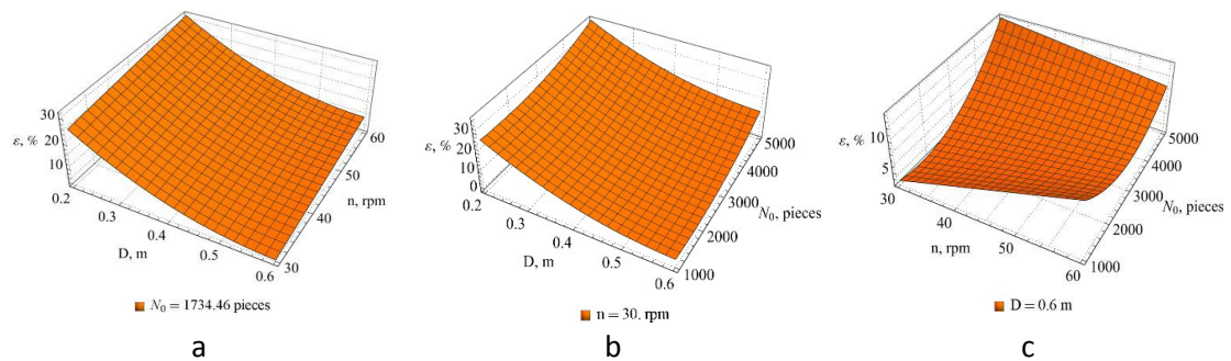
Fig. 14. The relative content of impurity elements \epsilon in the seed mixture, which was within the minimum \vartheta_{min} and maximum \vartheta_{max} rotation angles of the cylindrical cellules trier cylinder, depends on the diameter of the trier cylinder D , the rotation frequency of the trier cylinder n , and the number of seeds and impurities in the seed mixture N_0
