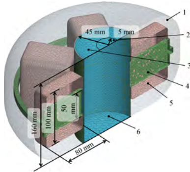
Fig. 1. 3D model of the main areas and elements of the vortex layer apparatus: 1 – inductor housing with transformer oil; 2 – working chamber; 3 – coil core; 4 – inductor coils
