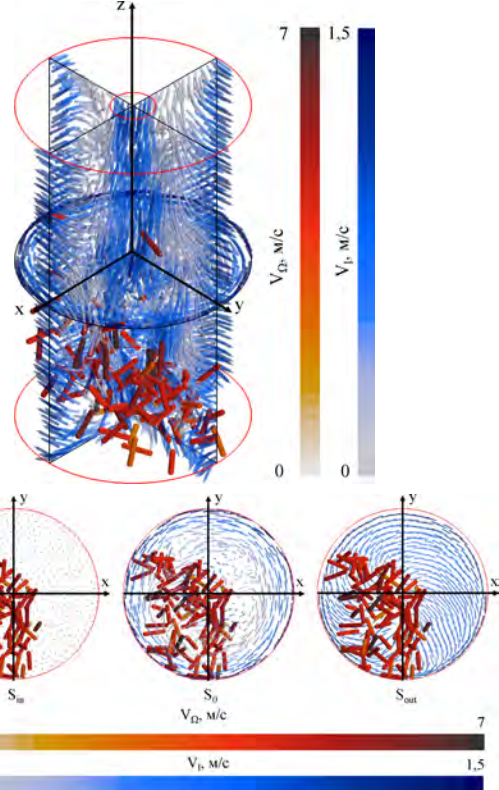
Fig. 14. Distribution of fluid and ferromagnet velocities in the working chamber of the vortex layer apparatus in rotating electromagnetic field
