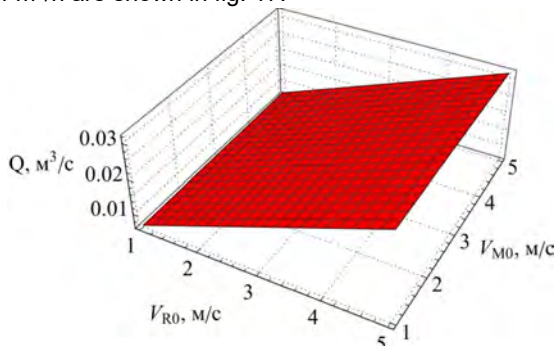
Fig. 17. Dependence between the vortex layer apparatus's volumetric productivity Q and the initial rate of liquid manure supply V_{R0} and the initial rate of the additional component supply V_{M0}
