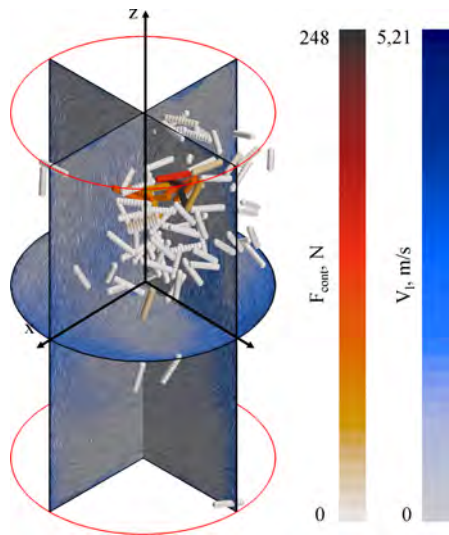
Fig. 7. Visualization of distribution of ferromagnets' contact interaction force F_{cont} under the action of rotating electromagnetic field in STAR-CCM+
