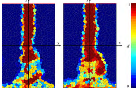
Fig. 12. Longitudinal sections of the working chamber of the vortex layer apparatus in a rotating electromagnetic field
