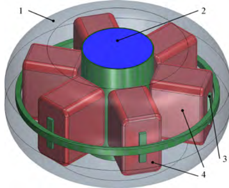
Fig. 2. Grid model of the vortex layer apparatus's main areas and elements: 1 – inductor housing area; 2 – additional component supply hole; 3 – mixture supply hole; 4 – coil core region; 5 – inductor coil area; 6 – working chamber area
