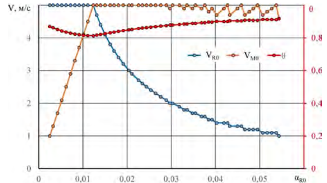
Fig. 18. Nomogram for calculating the initial rate of liquid manure supply V_{R0} and the initial rate of the additional component supply V_{M0} depending on the required share of additional components \alpha_{R0}
