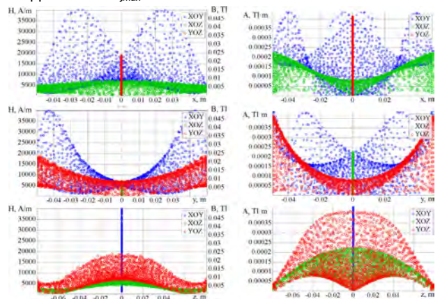
Fig. 4. Dependencies between electromagnetic indicators in the working chamber of the vortex layer apparatus and coordinates for accepted value of the magnetomotive force of only two opposite coils \xi_{\max} = 5000 \text{ A}\cdot\text{turns}
