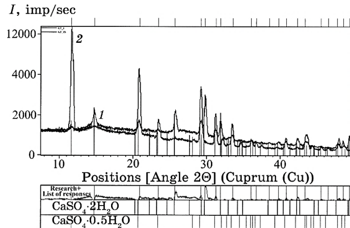
Fig. 4. Rietveld diagram of gypsum hardening over time for G-5: 1—after the 1 st cycle; 2—after the 18 th cycle.
