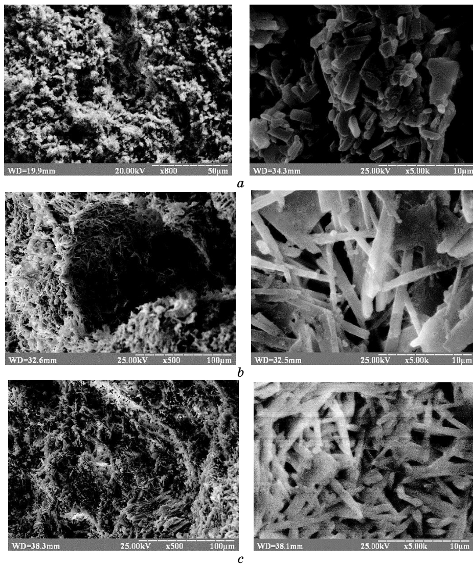
Fig. 11. Photomicrographs of the gypsum plaster structure: a ) gypsum plaster; b ) gypsum modified with pure CNTs; c ) gypsum modified with hydroxyl groups.
