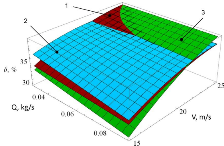
Fig. 7 – The dependence of the distribution coefficient \delta on the seeds supply Q and air flow velocity V
