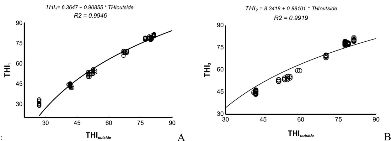
Fig. 1. Dependence of the temperature-humidity index (THI) in the barn of hangar type (A, THI_1 ) and in the barn of frame type (B, THI_2 ) on the THI value outside the buildings ( THI_{outside} ).
