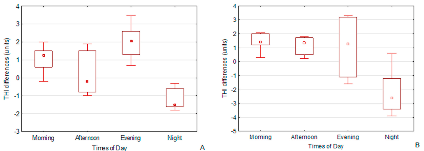
Fig. 3. Differences between the temperature-humidity index (THI) data provided by weather stations and the measured data outside the barn of hangar type (A) and of frame type with insulated roof (B) on one summer day in August and June during the verification study, respectively.
