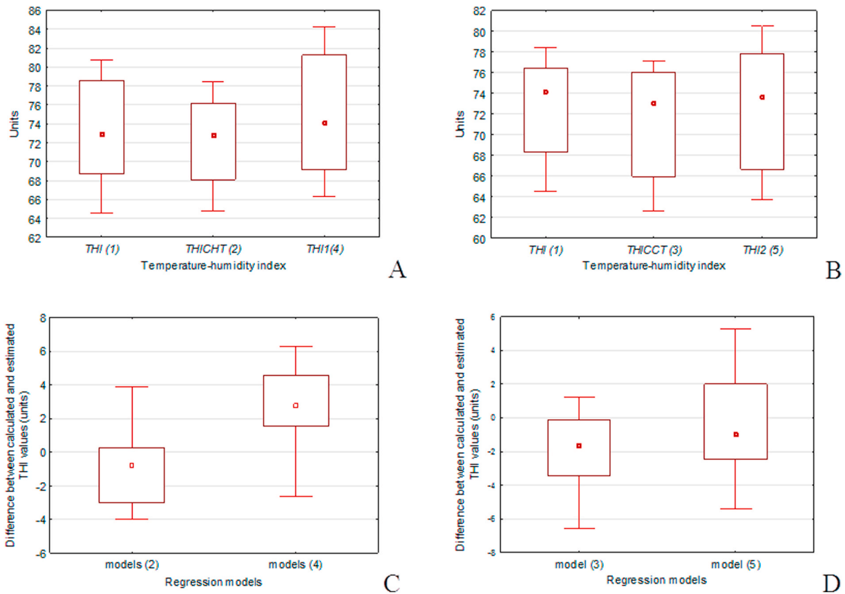
Fig. 2. Temperature-humidity index (THI) calculated with formula (1) according to Kibler (1964) and estimated with models (2) and (4) for the barn of hangar type (A) and with models (3) and (5) for the barn of frame type (B) with insulated roof. Differences between calculated and estimated THI values of models (2) and (4) for the barn of hangar type (C) and models (3) and (5) for the barn of frame type with insulated roof (D).
